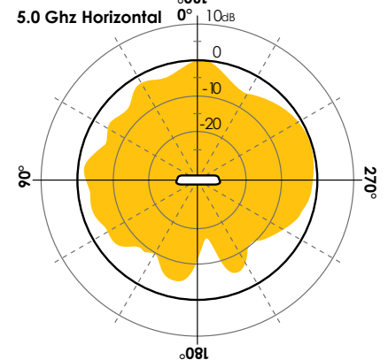
5.0 Ghz Horizontal
