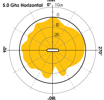
5.0 Ghz Horizontal
