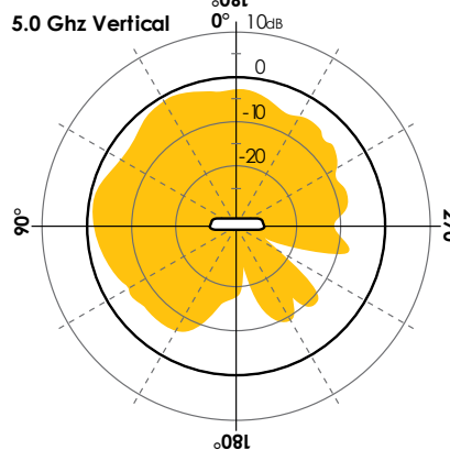
5.0 Ghz Vertical
